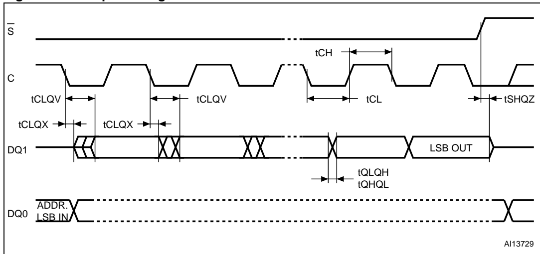
Figure 33. Output timing
