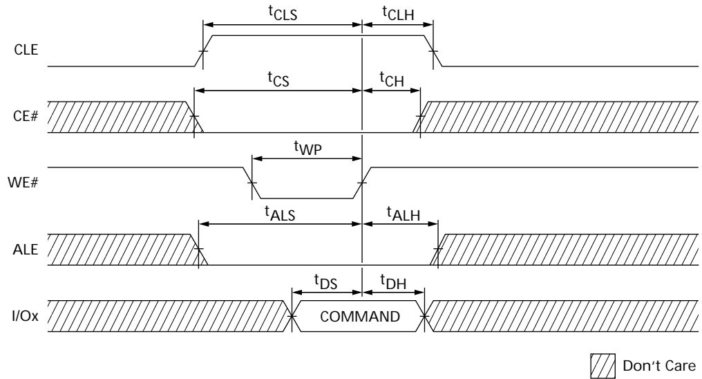
Figure 44: COMMAND LATCH Cycle
