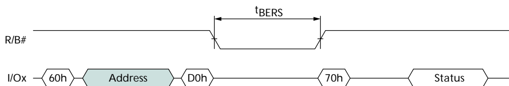
Figure 24: BLOCK ERASE Operation
