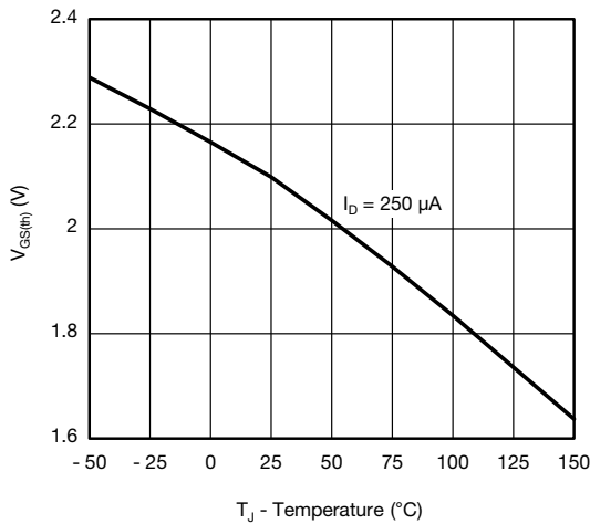
Threshold Voltage
