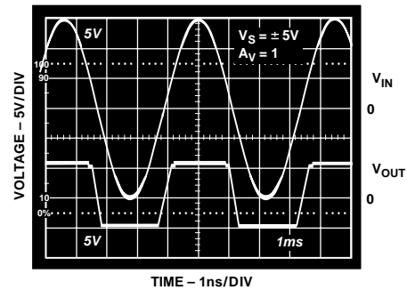
Figure 2. Output Voltage Phase Reversal Behavior
