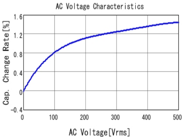
■ DE11XRA150KN4AQ01F C-AC Voltage capchange, DCOV, 20.0
