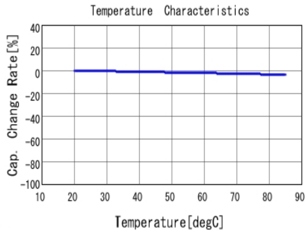
■ DE11XRA150KN4AQ01F C-Temp. capchange, DCOV, AC1Vrms
