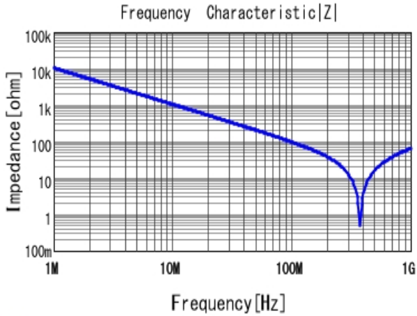
■ DE11XRA150KN4AQ01F |Z| DCOV, 20degC
