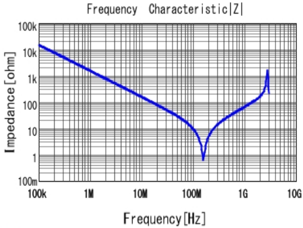
■ DE2B3KY151KN2AM01F |Z| DCOV, 20degC
