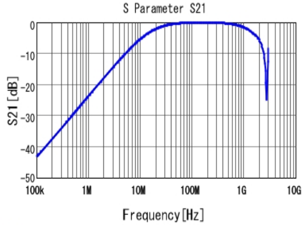
■ DE2B3KY151KN2AM01F S21 DCOV, 20degC
