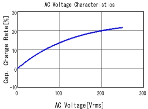
■ DE2B3KY151KN2AM01F C-AC Voltage capchange, DCOV, 20.0
