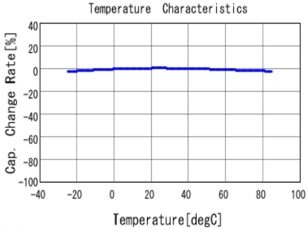
■ DE2B3KY151KN2AM01F C-Temp. capchange, DCOV, AC1Vrms
