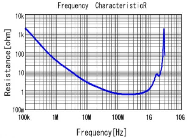
■ DE2B3KY151KN2AM01F R DCOV, 20degC
