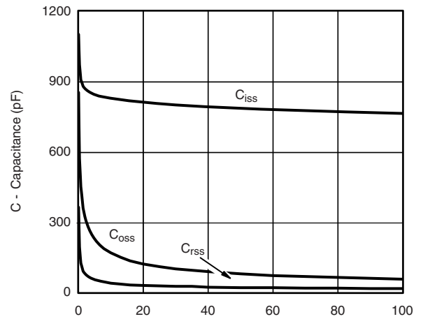
V_{DS} - Drain-to-Source Voltage Capacitance
