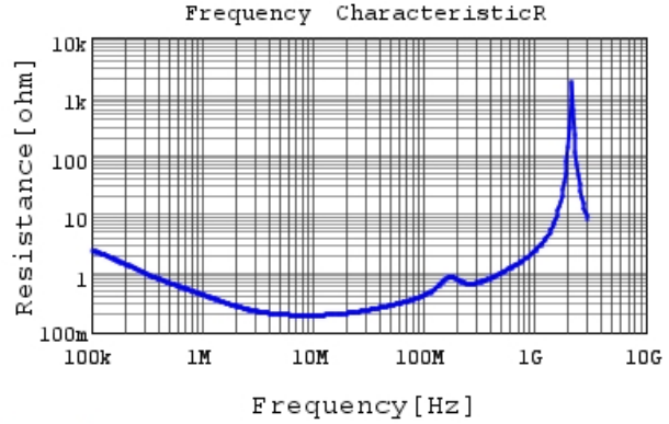
DE2F3KY103MA3BM02F R DCOV, 20degC
