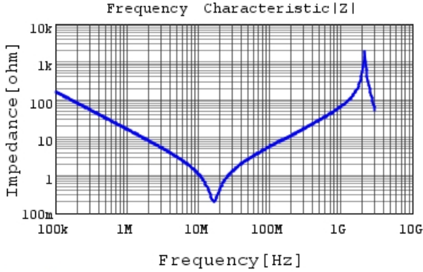
DE2F3KY103MA3BM02F |Z| DCOV, 20degC
