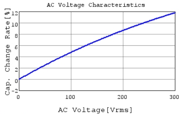
DE1B3KX101KA4BP01F C-AC Voltage capchange, I
