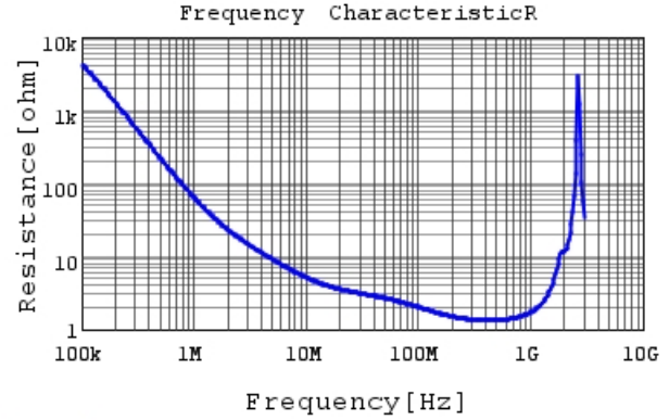
DE1B3KX101KA4BP01F R DC0V, 20degC
