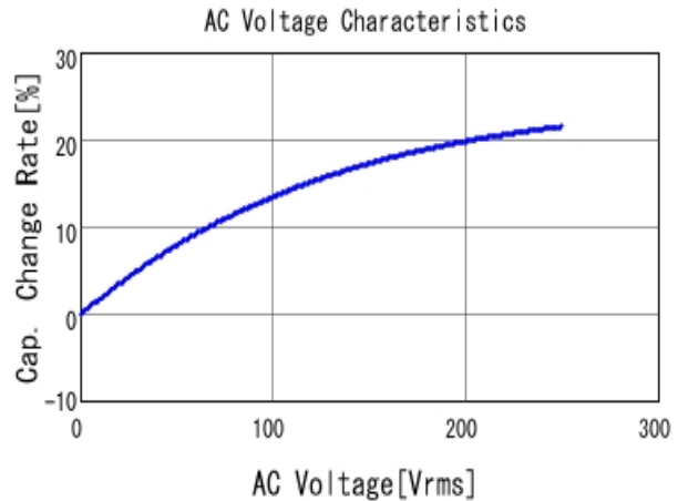
■ DE2B3KY151KA2BM01F C-AC Voltage capchange, DCOV, 20.0
