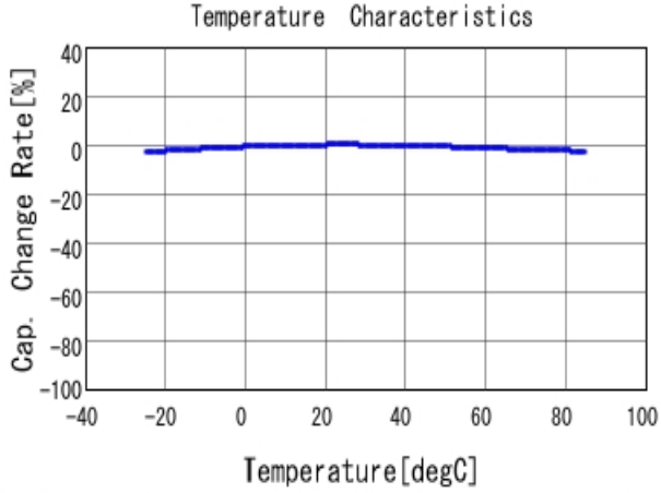
■ DE2B3KY151KA2BM01F C-Temp. capchange, DCOV, AC1Vrms
