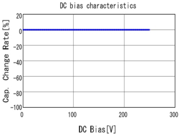
■ DE2B3KY151KA2BM01F C-DC bias capchange, 20.0degC, AC1
