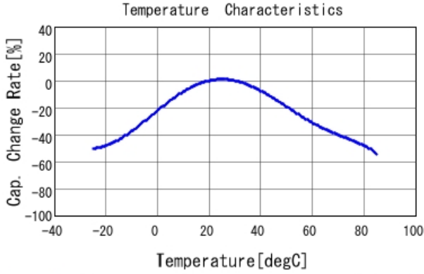
DE1E3RA152MN4AP01F C-Temp. capchange, DCOV, AC1Vrrr
