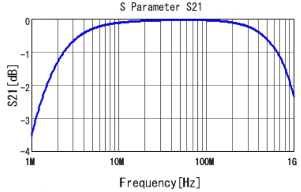
DE1E3RA152MN4AP01F S21 DCOV, 20degC
