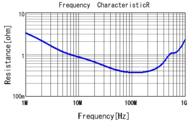
DE1E3RA152MN4AP01F R DC0V, 20degC
