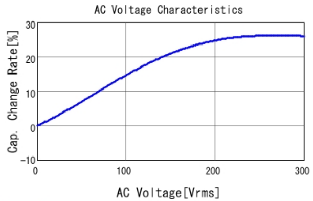
DE1E3RA152MN4AP01F C-AC Voltage capchange, DC0V, 2
