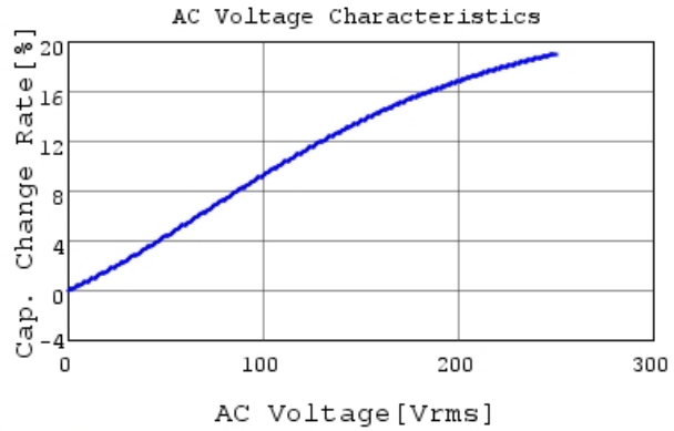
DE2B3SA151KJ3BT02F C-AC Voltage capchange, I
