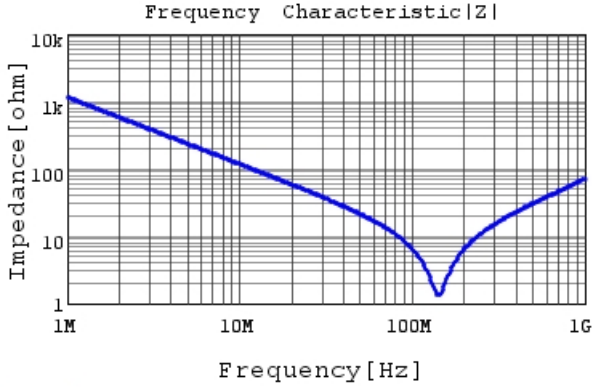
DE2B3SA151KJ3BT02F |Z| DC0V, 20degC
