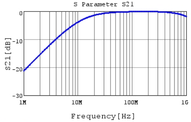
DE2B3SA151KJ3BT02F S21 DCOV, 20degC
