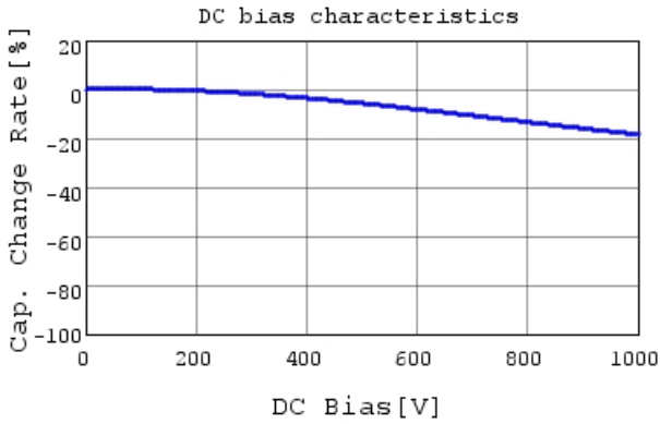
DE2B3SA151KJ3BT02F C-DC bias capchange, 20.0
