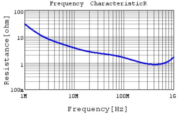
DE2B3SA151KJ3BT02F R DC0V, 20degC
