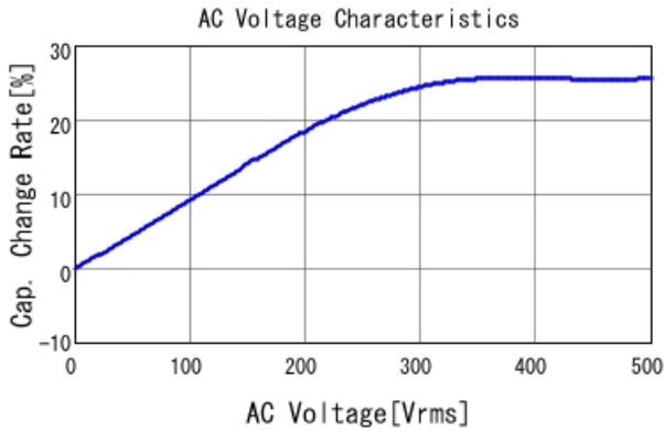
DE1E3RB222MJ4BR01F C-AC Voltage capchange, DCOV, 2
