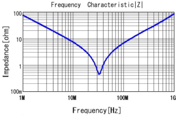
DE1E3RB222MJ4BR01F |Z| DCOV, 20degC
