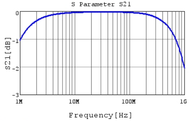
DE2E3SA332MJ3BT02F S21 DCOV, 20degC
