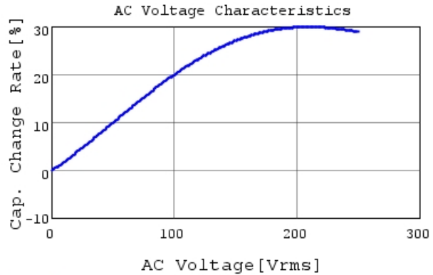
DE2E3SA332MJ3BT02F C-AC Voltage capchange, I
