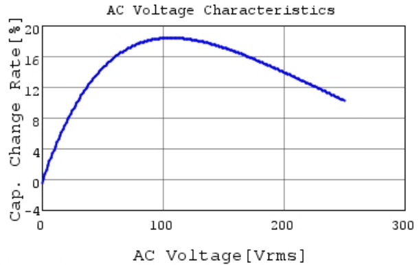
DE2F3KY103MN3AM02F C-AC Voltage capchange, I
