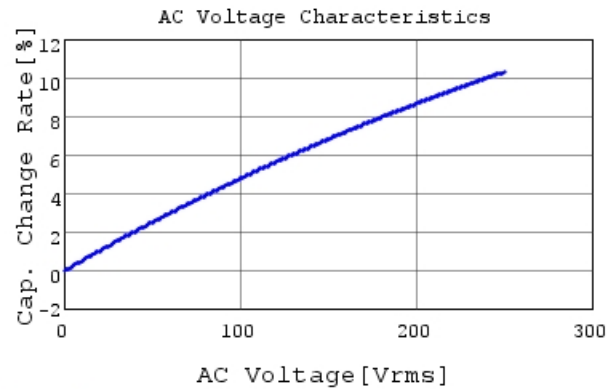
DE1B3KX101KN4AN01F C-AC Voltage capchange, I
