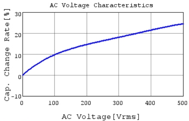
DE1B3RA331KJ4BQ01F C-AC Voltage capchange, I
