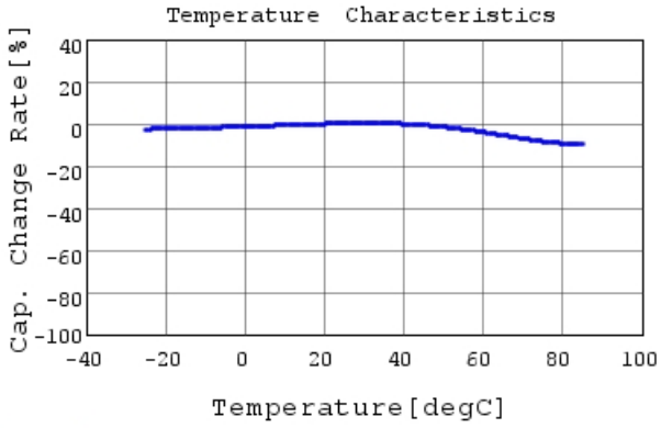
DE1B3RA331KJ4BQ01F C-Temp. capchange, DCOV,
