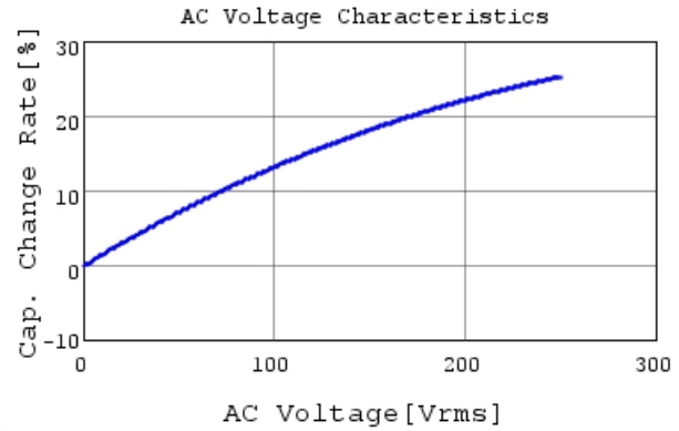
DE1E3KX152MN4AN01F C-AC Voltage capchange, I
