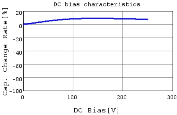
DE1E3KX152MN4AN01F C-DC bias capchange, 20.0
