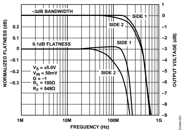
Figure 32. -3 dB Bandwidth vs. Frequency, G = -1
