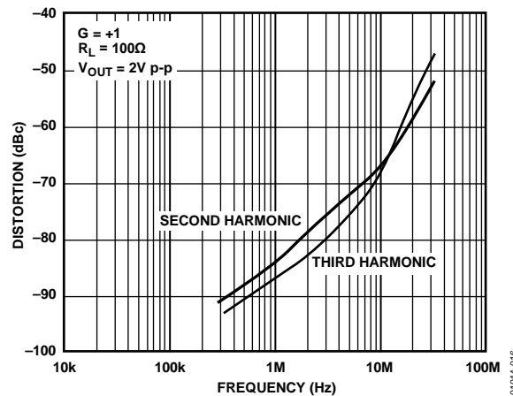
Figure 17. Distortion vs. Frequency, G = +1 , R_L = 100\ \Omega
