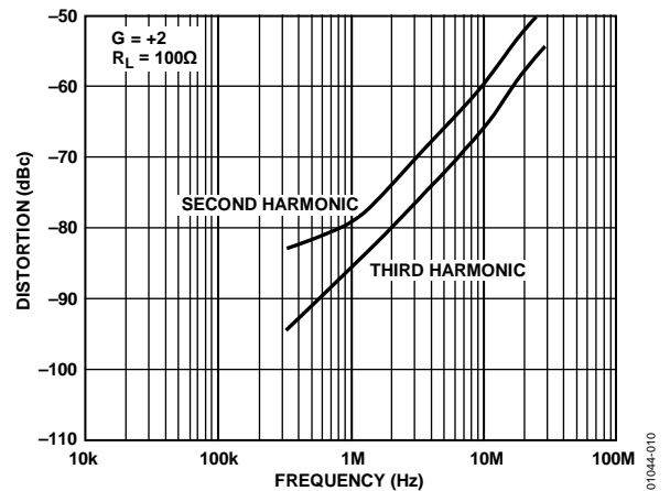
Figure 11. Distortion vs. Frequency, G = +2 , R_L = 100 \Omega
