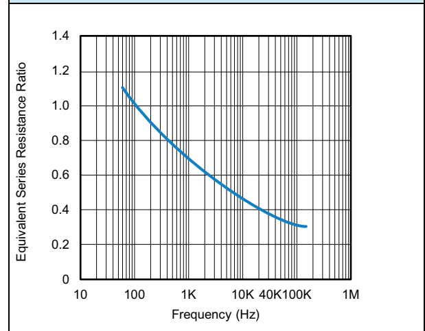
TYP. ESR AS A FUNCTION OF FREQUENCY
