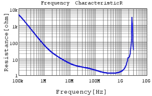
DE1B3KX101KJ4BP01F R DC0V, 20degC
