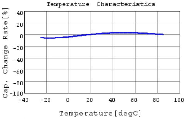
DE1B3KX101KJ4BP01F C-Temp. capchange, DCOV,
