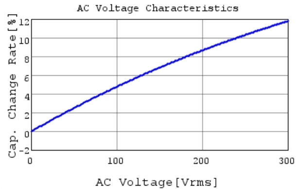
DE1B3KX101KJ4BP01F C-AC Voltage capchange, I
