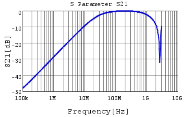
DE1B3KX101KJ4BP01F S21 DCOV, 20degC
