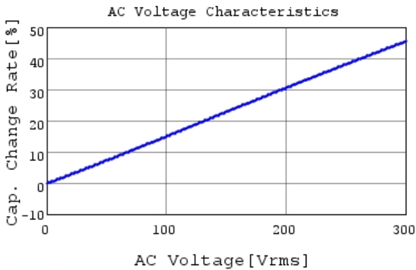
DE6B3KJ331KN3A C-AC Voltage capchange, DCOV,
