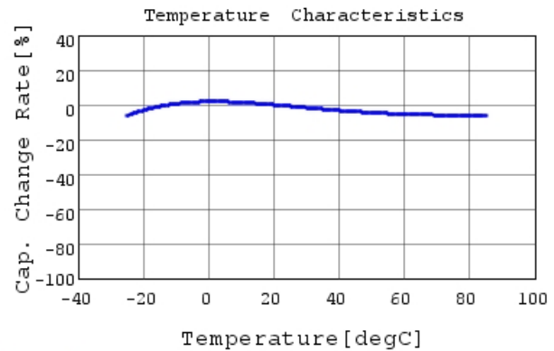
DE6B3KJ331KN3A C-Temp. capchange, DCOV, AC1V
