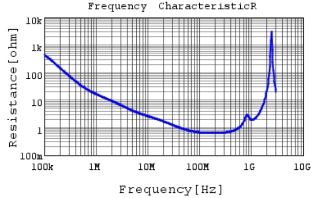
DE6B3KJ331KN3A R DCOV, 20degC
