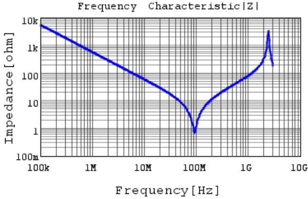
DE6B3KJ331KN3A |Z| DCOV, 20degC
