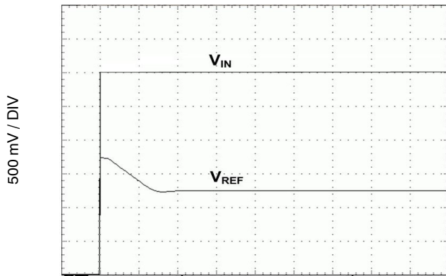
Figure 14. Turn-On Time
