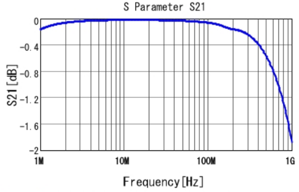
DE2E3SA103MA3BT02F S21 DCOV, 20degC
