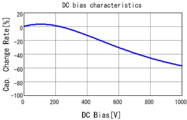
DE2E3SA103MA3BT02F C-DC bias capchange, 20.0degC,
