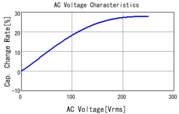
DE2E3SA103MA3BT02F C-AC Voltage capchange, DC0V, 2
