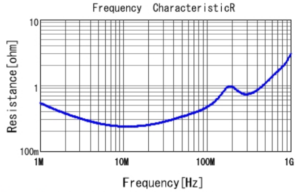
DE2E3SA103MA3BT02F R DC0V, 20degC
