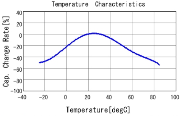
DE2E3SA103MA3BT02F C-Temp. capchange, DCOV, AC1Vrrr
