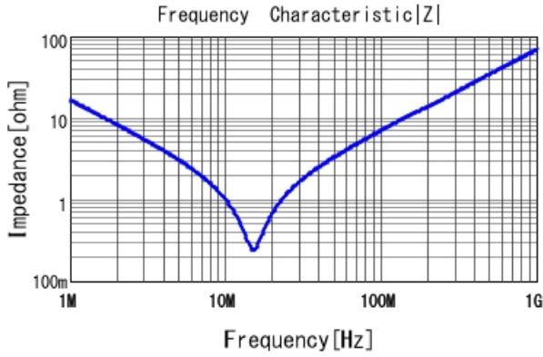
DE2E3SA103MA3BT02F |Z| DC0V, 20degC
