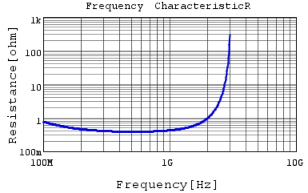
DE21XKY100JA3BM02F R DCOV, 20degC
