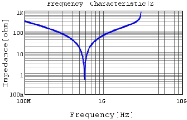
DE21XKY100JA3BM02F |Z| DCOV, 20degC
