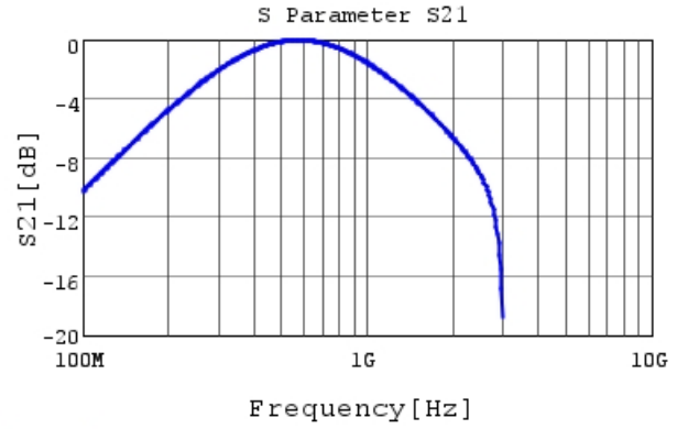
DE21XKY100JA3BM02F S21 DCOV, 20degC
