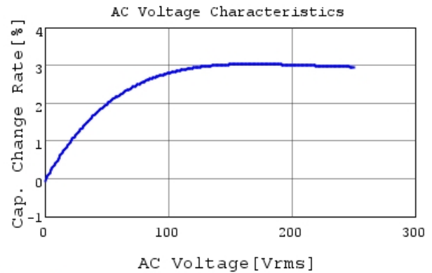
DE21XKY100JA3BM02F C-AC Voltage capchange, I
