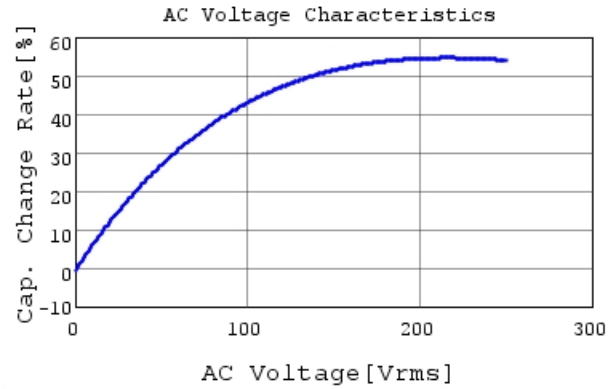
DE2E3KY222MA2BM01F C-AC Voltage capchange, I
