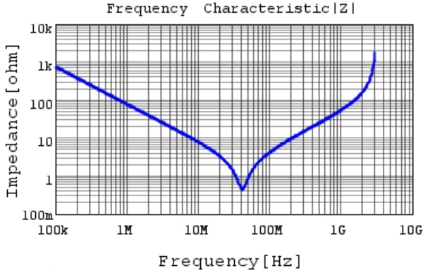
DE2E3KY222MA2BM01F |Z| DCOV, 20degC
