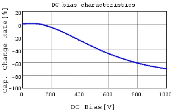
DE2E3SA332MA3BT02F C-DC bias capchange, 20.0
