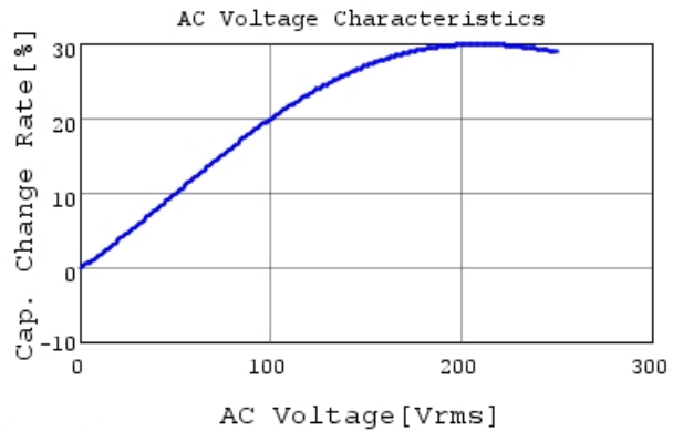
DE2E3SA332MA3BT02F C-AC Voltage capchange, I
