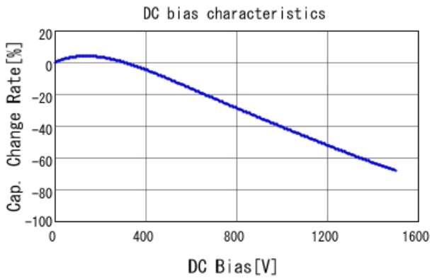
DE2E3SA472MJ3BY02F C-DC bias capchange, 20.0degC,
