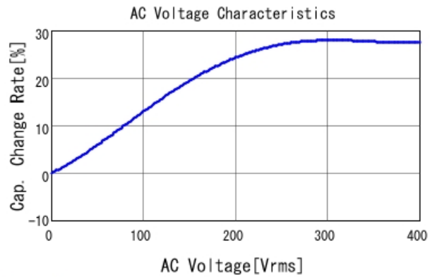
DE2E3SA472MJ3BY02F C-AC Voltage capchange, DC0V, 2
