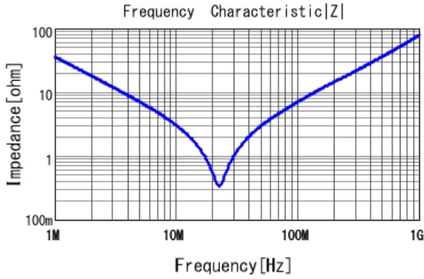
DE2E3SA472MJ3BY02F |Z| DC0V, 20degC
