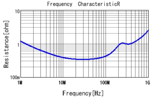
DE2E3SA472MJ3BY02F R DC0V, 20degC
