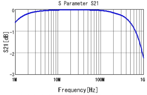
DE2E3SA472MJ3BY02F S21 DCOV, 20degC
