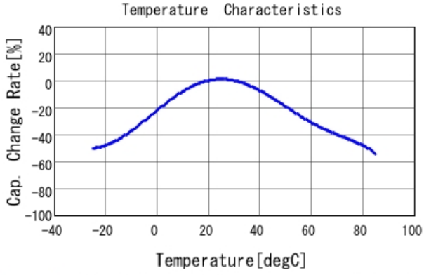
DE2E3SA472MJ3BY02F C-Temp. capchange, DCOV, AC1Vrrr
