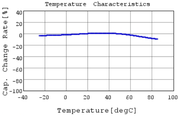
DE1B3KX681KA4BP01F C-Temp. capchange, DCOV,
