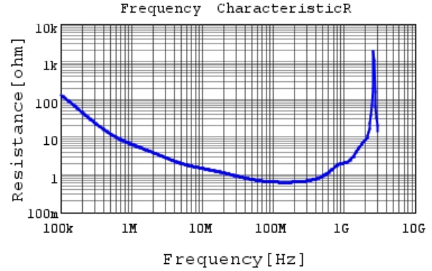
DE1B3KX681KA4BP01F R DCOV, 20degC
