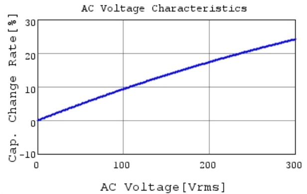
DE1B3KX681KA4BP01F C-AC Voltage capchange, I
