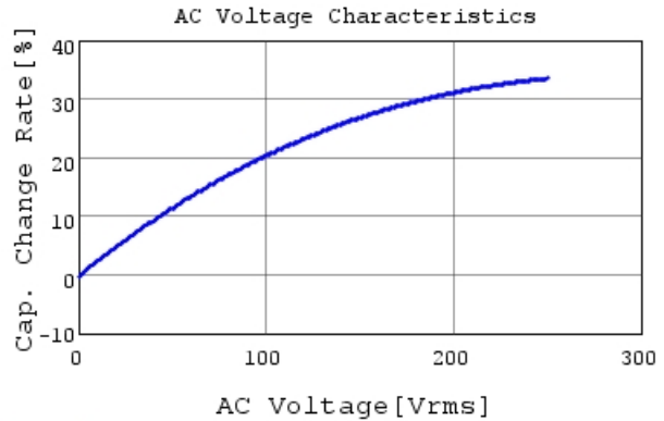
DE2E3KY332MB3BM02F C-AC Voltage capchange, I
