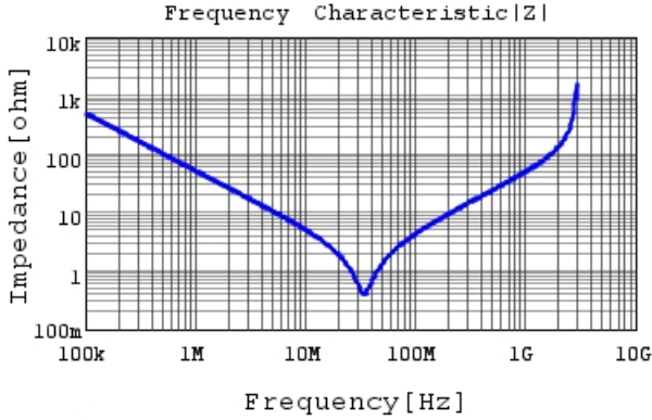
DE2E3KY332MB3BM02F |Z| DC0V, 20degC
