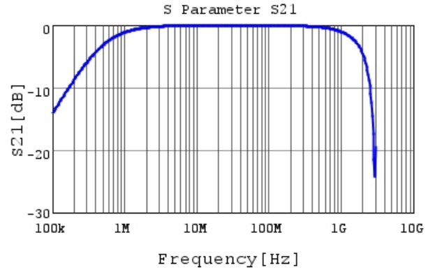
DE2E3KY332MB3BM02F S21 DCOV, 20degC
