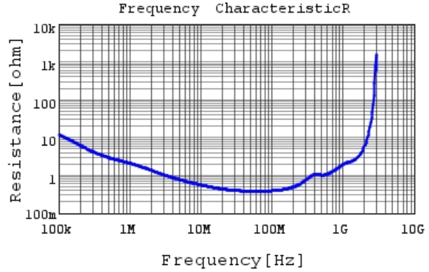
DE2E3KY332MB3BM02F R DC0V, 20degC
