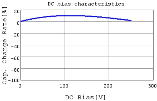
DE2E3KY332MB3BM02F C-DC bias capchange, 20.0
