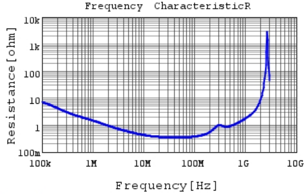
DE2E3KY472MA2BM01F R DC0V, 20degC
