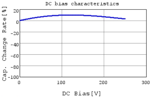
DE2E3KY472MA2BM01F C-DC bias capchange, 20.0
