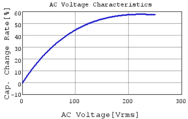
DE2E3KY472MA2BM01F C-AC Voltage capchange, I
