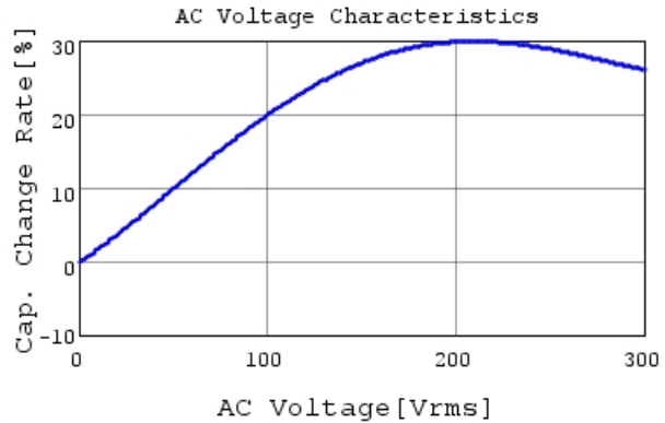
DE2E3SA332MA3BX02F C-AC Voltage capchange, I
