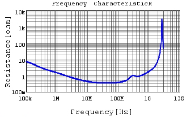
DE2E3KY472MB3BU02F R DC0V, 20degC
