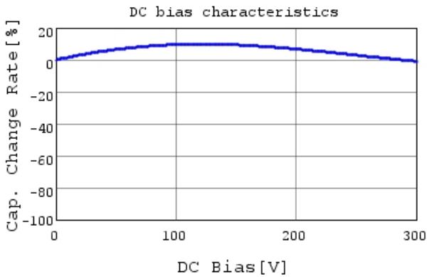
DE2E3KY472MB3BU02F C-DC bias capchange, 20.0
