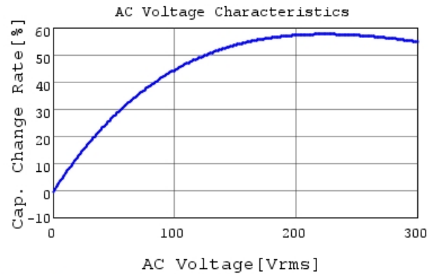
DE2E3KY472MB3BU02F C-AC Voltage capchange, I
