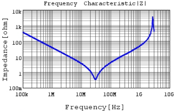
DE2E3KY472MB3BU02F |Z| DC0V, 20degC
