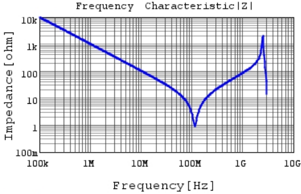
DE1B3KX221KA4BP01F |Z| DC0V, 20degC
