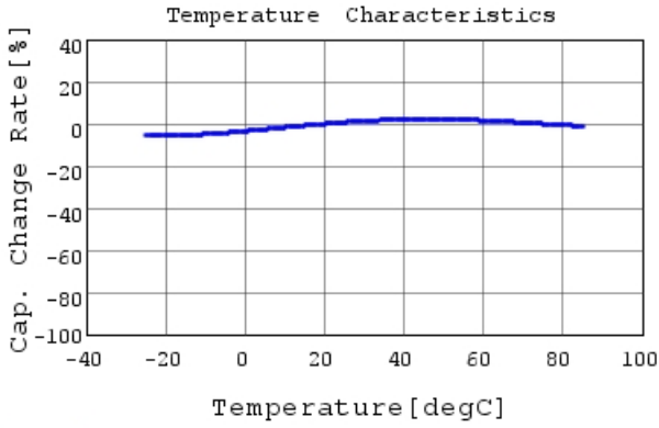
DE1B3KX221KA4BP01F C-Temp. capchange, DCOV,
