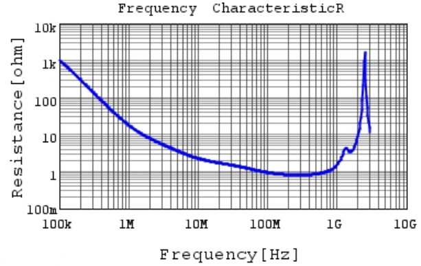
DE1B3KX221KA4BP01F R DC0V, 20degC
