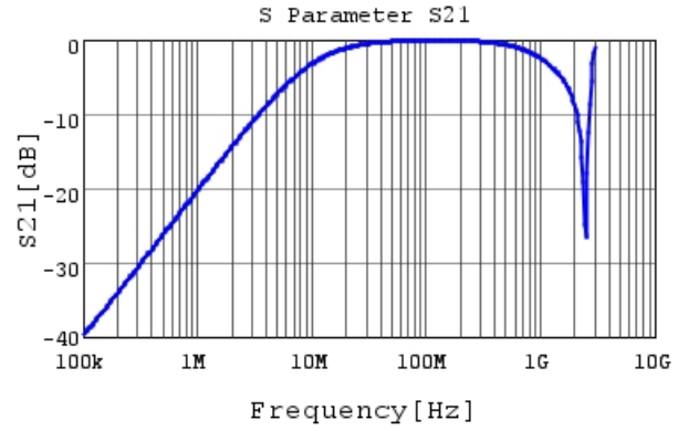
DE1B3KX221KA4BP01F S21 DCOV, 20degC
