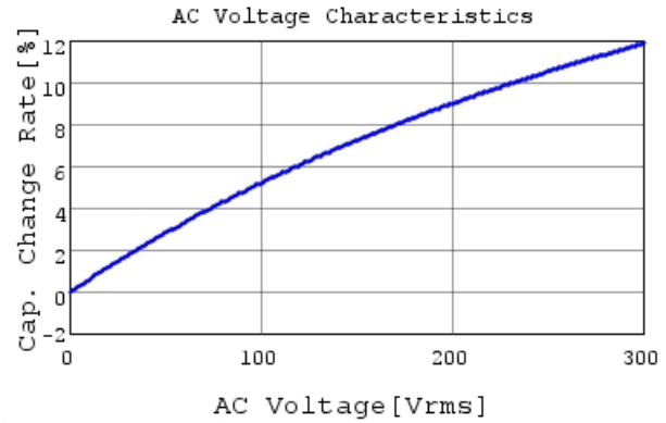
DE1B3KX221KA4BP01F C-AC Voltage capchange, I
