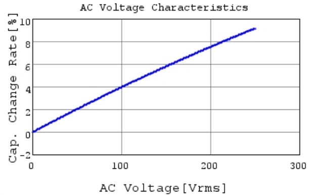
DE1B3KX151KN4AN01F C-AC Voltage capchange, I
