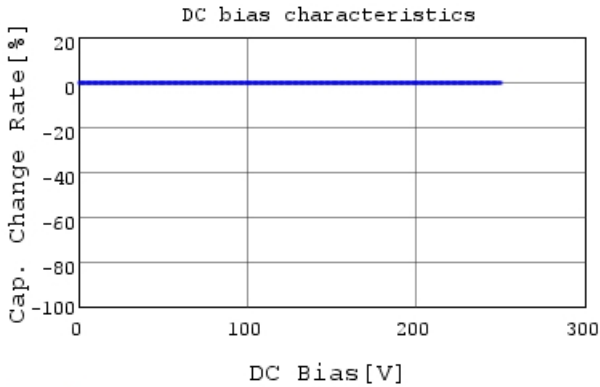
DE1B3KX151KN4AN01F C-DC bias capchange, 20.0
