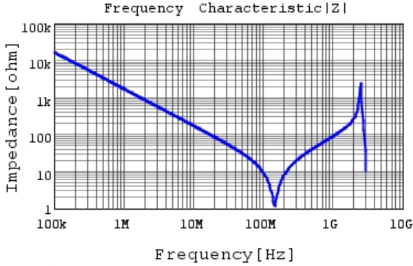
DE1B3KX151KN4AN01F |Z| DCOV, 20degC
