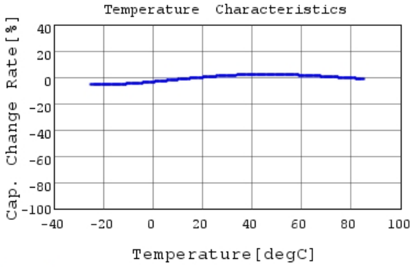
DE1B3KX151KN4AN01F C-Temp. capchange, DCOV,
