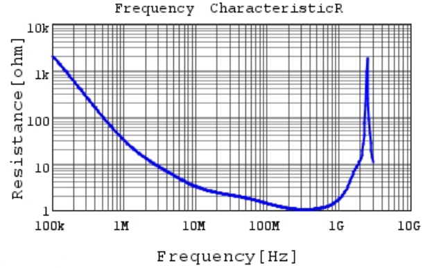
DE1B3KX151KN4AN01F R DCOV, 20degC
