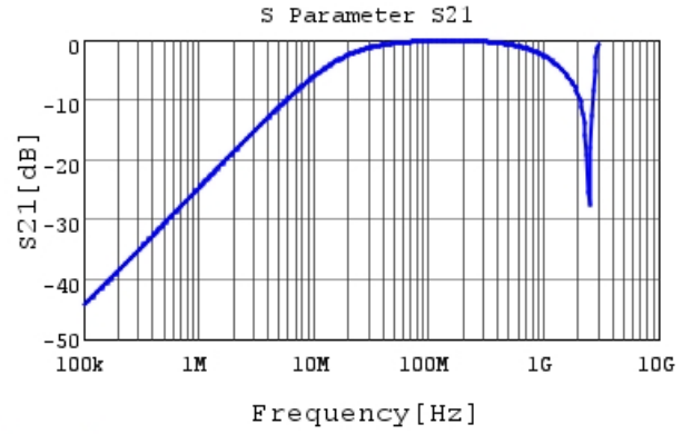
DE1B3KX151KN4AN01F S21 DCOV, 20degC
