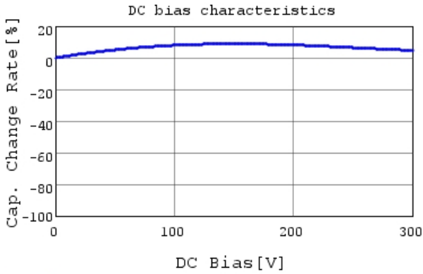
DE2E3KY102MB3BU02F C-DC bias capchange, 20.0
