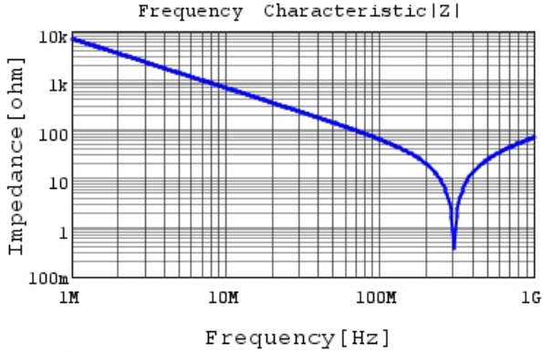
DE11XRA220KN4AQ01F |Z| DCOV, 20degC
