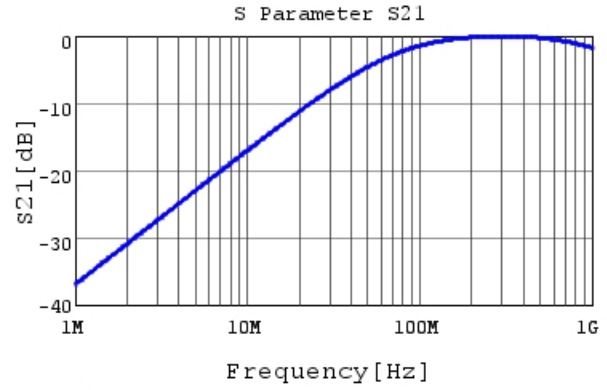
DE11XRA220KN4AQ01F S21 DCOV, 20degC
