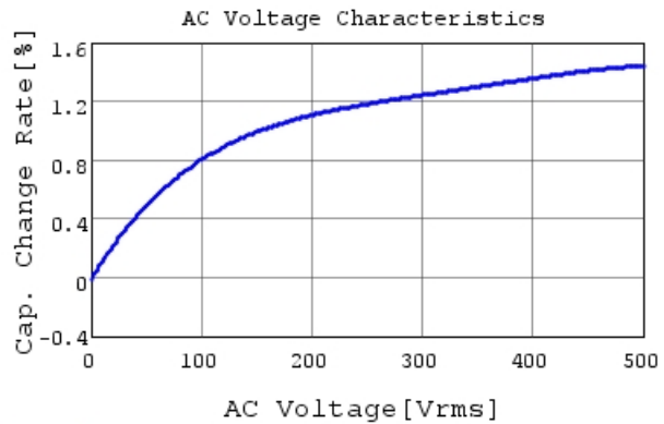
DE11XRA220KN4AQ01F C-AC Voltage capchange, I
