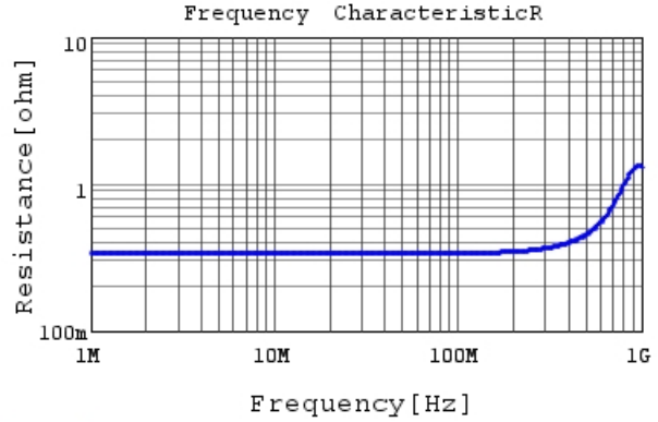
DE11XRA220KN4AQ01F R DCOV, 20degC
