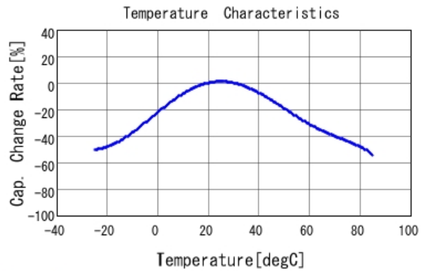
DE1E3RA152MA4BN01F C-Temp. capchange, DCOV, AC1Vrr
