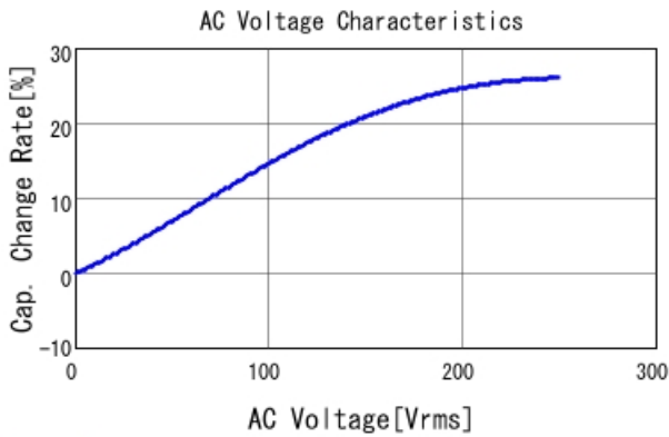
DE1E3RA152MA4BN01F C-AC Voltage capchange, DCOV, 2
