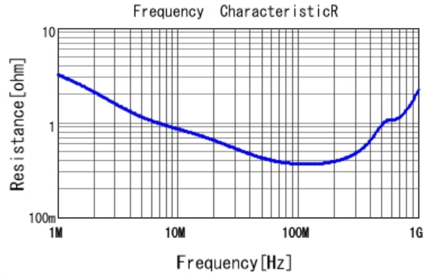
DE1E3RA152MA4BN01F R DCOV, 20degC
