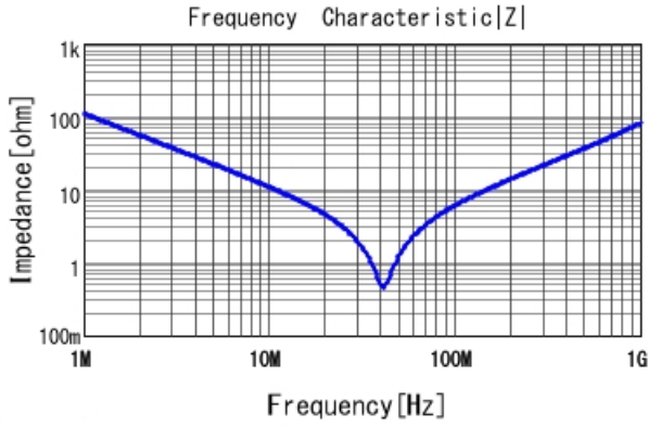
DE1E3RA152MA4BN01F |Z| DCOV, 20degC
