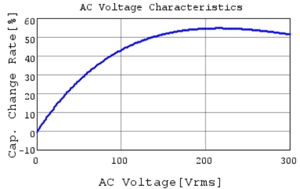
DE2E3KY222MN3AU02F C-AC Voltage capchange, I
