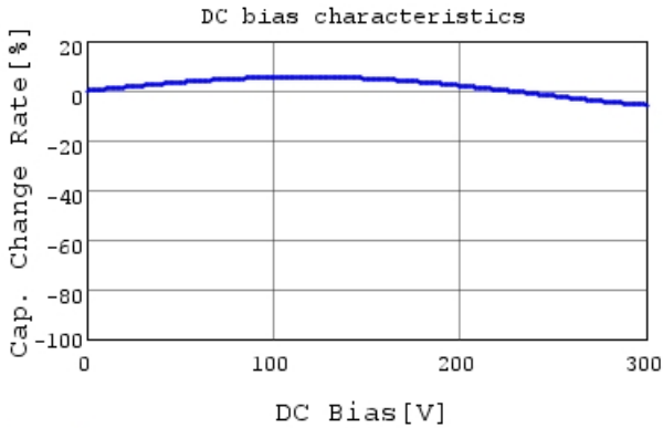
DE2E3KY222MN3AU02F C-DC bias capchange, 20.0
