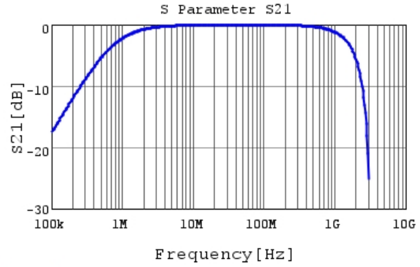
DE2E3KY222MN3AU02F S21 DCOV, 20degC
