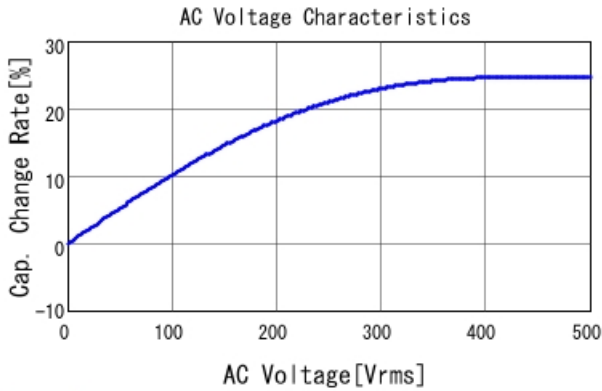
DE1E3RB332MN4AR01F C-AC Voltage capchange, DCOV, 2
