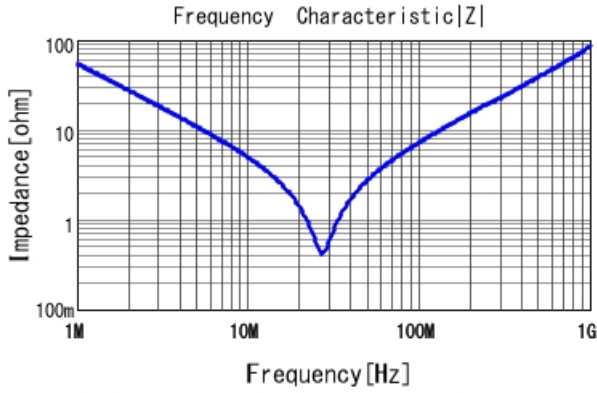
DE1E3RB332MN4AR01F |Z| DCOV, 20degC
