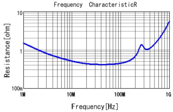
DE1E3RB332MN4AR01F R DCOV, 20degC
