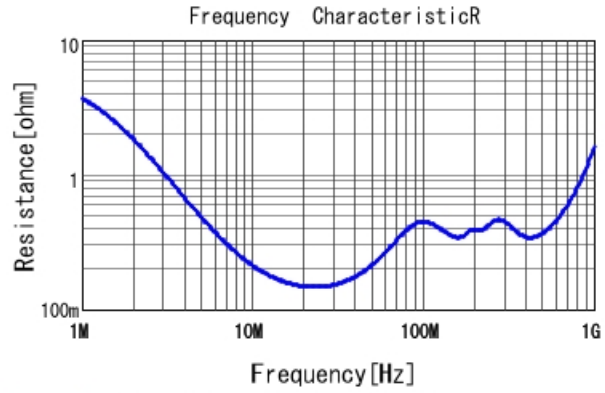
DE11XRA220KN4AN01F R DCOV, 20degC
