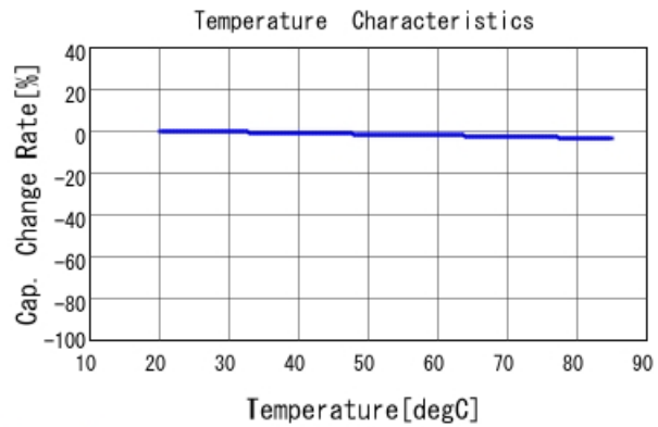
DE11XRA220KN4AN01F C-Temp. capchange, DCOV, AC1Vrr
