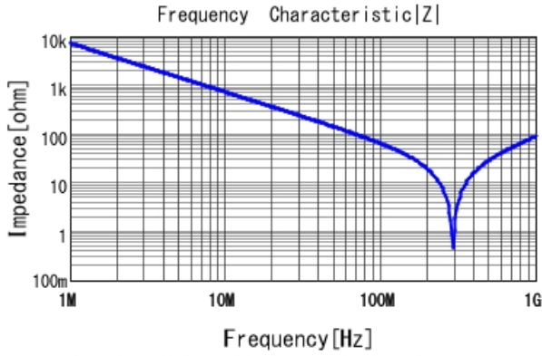
DE11XRA220KN4AN01F |Z| DCOV, 20degC
