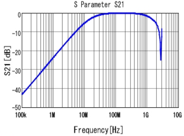
■ DE2B3KY151KB2BM01F S21 DCOV, 20degC
