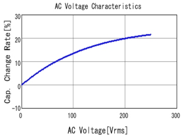
■ DE2B3KY151KB2BM01F C-AC Voltage capchange, DCOV, 20.0
