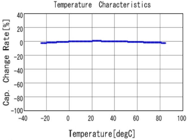
■ DE2B3KY151KB2BM01F C-Temp. capchange, DCOV, AC1Vrms
