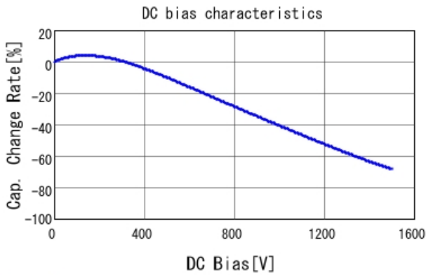
DE2E3SA332MN3AY02F C-DC bias capchange, 20.0degC,
