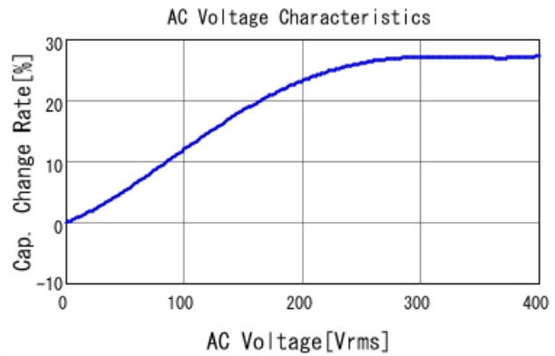
DE2E3SA332MN3AY02F C-AC Voltage capchange, DC0V, 2
