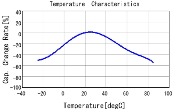
DE2E3SA332MN3AY02F C-Temp. capchange, DCOV, AC1Vrrr
