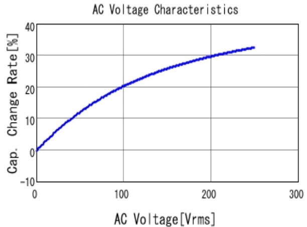
■ DE2B3KY221KN3AM02F C-AC Voltage capchange, DCOV, 20.0
