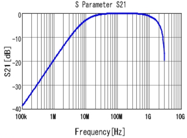
■ DE2B3KY221KN3AM02F S21 DCOV, 20degC
