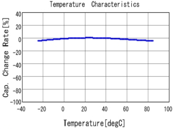
■ DE2B3KY221KN3AM02F C-Temp. capchange, DCOV, AC1Vrms
