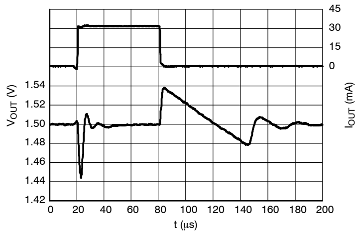
Figure 28. Load Transients, 1.5 V Version, I_{\text{OUT}} = 1 - 30 \text{ mA} , t_{\text{R}} = t_{\text{F}} = 0.5 \mu\text{s} , V_{\text{IN}} = 2.6 \text{ V}
