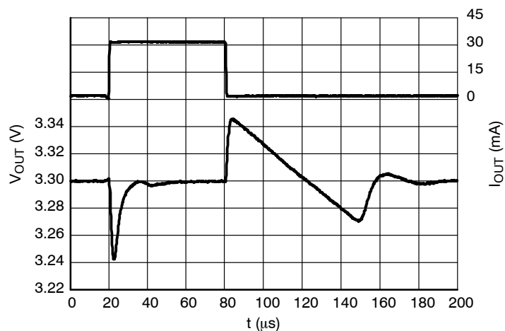
Figure 29. Load Transients, 3.3 V Version, I_{\text{OUT}} = 1 - 30 \text{ mA} , t_{\text{R}} = t_{\text{F}} = 0.5 \mu\text{s} , V_{\text{IN}} = 4.3 \text{ V}
