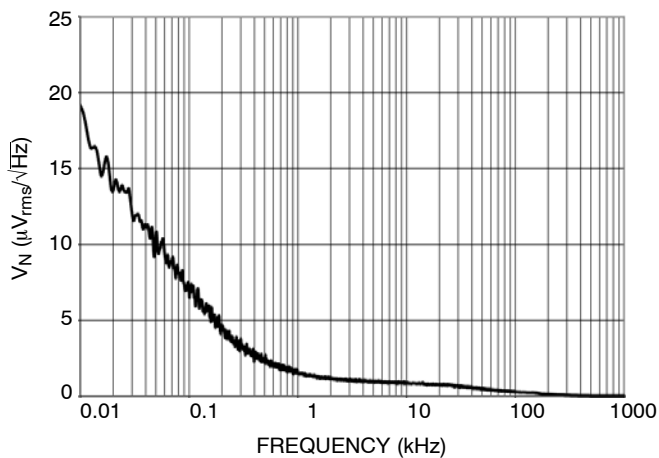
Figure 21. Output Voltage Noise, 5.0 V Version, V_{IN} = 6.0 \text{ V} , I_{OUT} = 30 \text{ mA}
