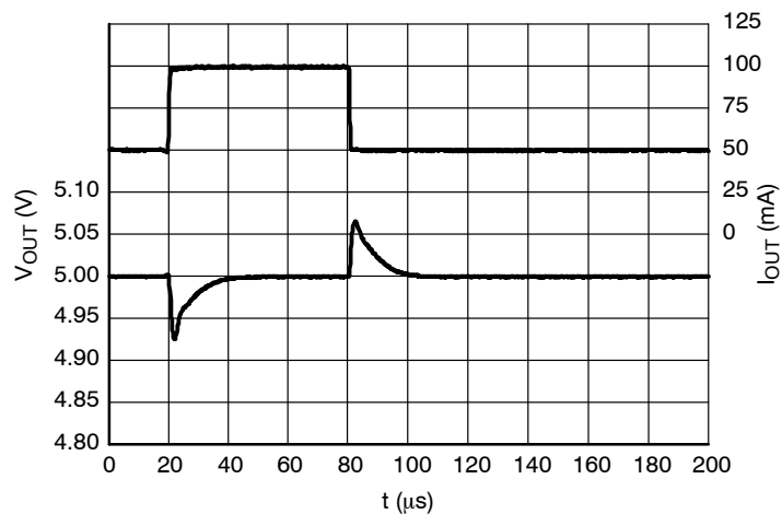
Figure 27. Load Transients, 5.0 V Version, I_{\text{OUT}} = 50 - 100 \text{ mA} , t_{\text{R}} = t_{\text{F}} = 0.5 \mu\text{s} , V_{\text{IN}} = 6.0 \text{ V}
