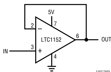
Rail-to-Rail Buffer
