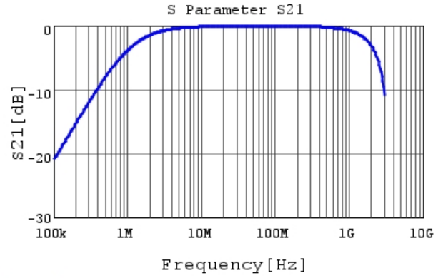
DE2E3KY152MA3BM02F S21 DCOV, 20degC
