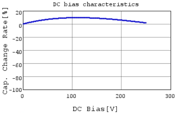
DE2E3KY152MA3BM02F C-DC bias capchange, 20.0
