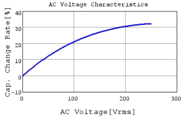
DE2E3KY152MA3BM02F C-AC Voltage capchange, I
