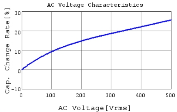
DE1B3RB221KJ4BR01F C-AC Voltage capchange, I
