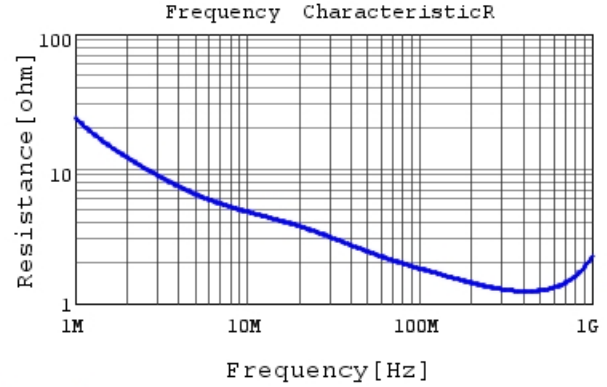
DE1B3RB221KJ4BR01F R DCOV, 20degC
