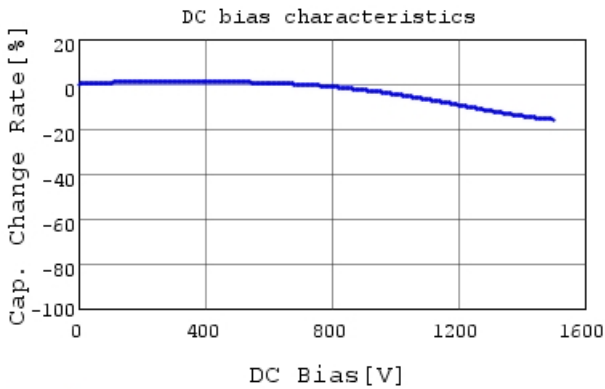
DE1B3RB221KJ4BR01F C-DC bias capchange, 20.0
