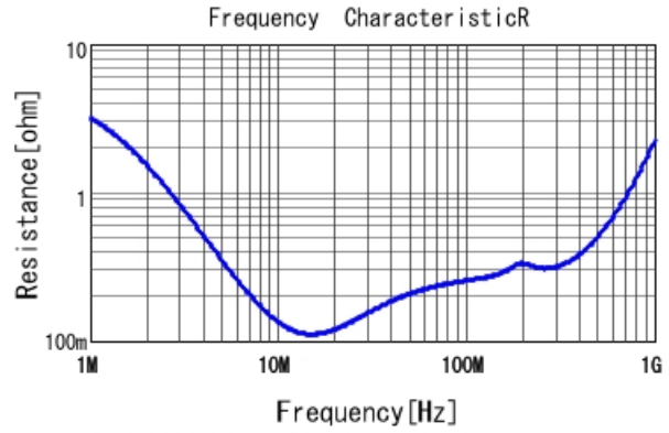
DE11XRA680KN4AP01F R DCOV, 20degC
