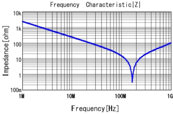
DE11XRA680KN4AP01F |Z| DCOV, 20degC
