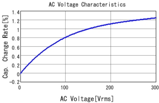
DE11XRA680KN4AP01F C-AC Voltage capchange, DCOV, 2
