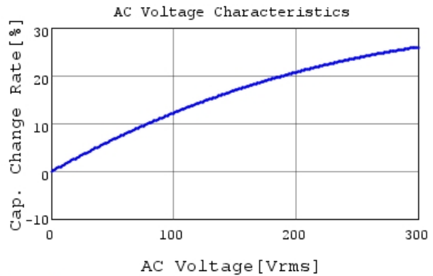
DE1E3KX332MN4AP01F C-AC Voltage capchange, I
