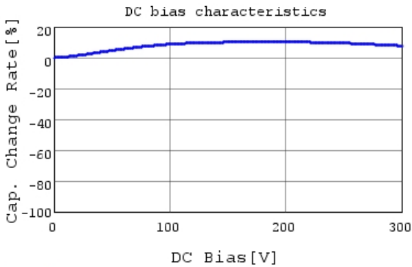
DE1E3KX332MN4AP01F C-DC bias capchange, 20.0
